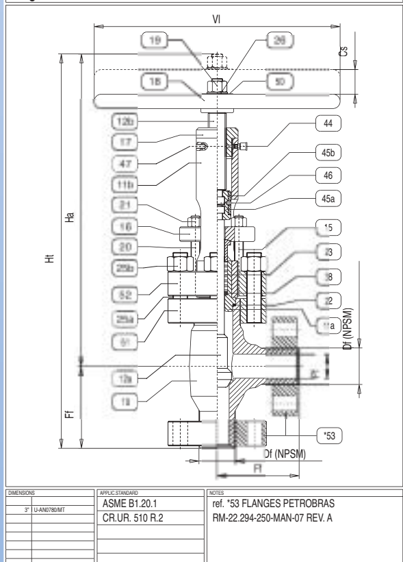
Angle block valve UREA service P.N. 325 Male threaded NPSM
