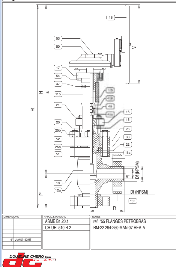
Angle block valve UREA service P.N. 325 Male threaded NPSM
