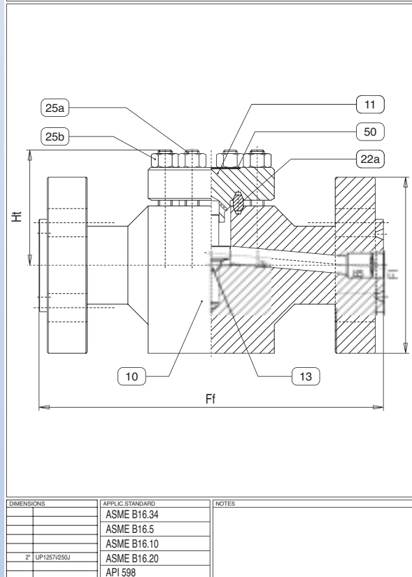
Piston check UREA SERVICE - 2500 - Full B. - Bolted - RJ
